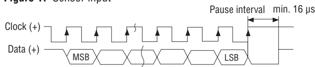
Figure 2. Timing Diagram
